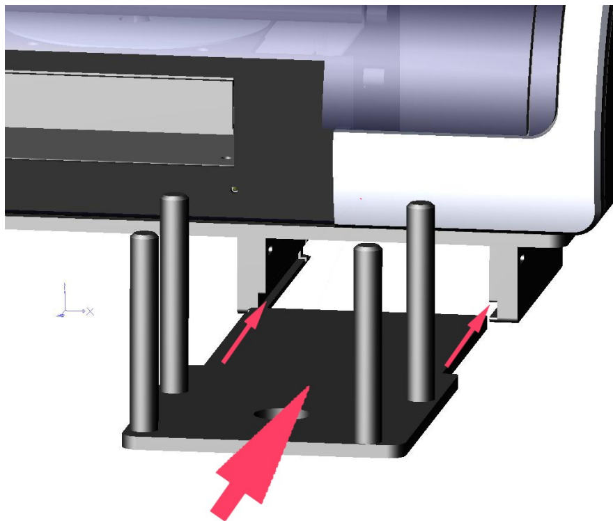
Fig. 3 Mounting the CD/DVD output tray
